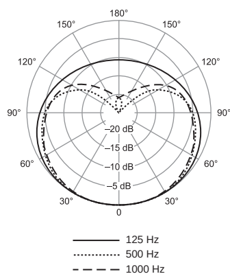
TYPICAL POLAR PATTERNS
