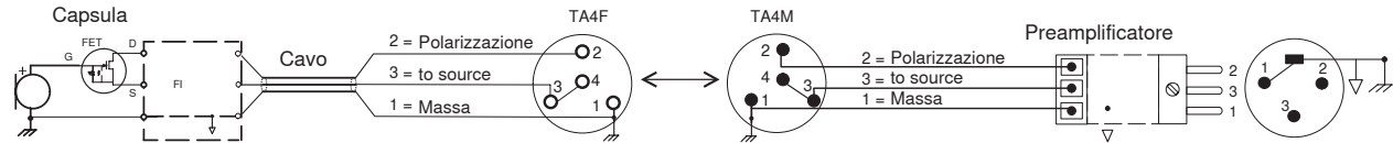
Schema circuitale
